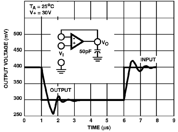
FIGURE 8. VOLTAGE FOLLOWER PULSE RESPONSE (SMALL SIGNAL)
